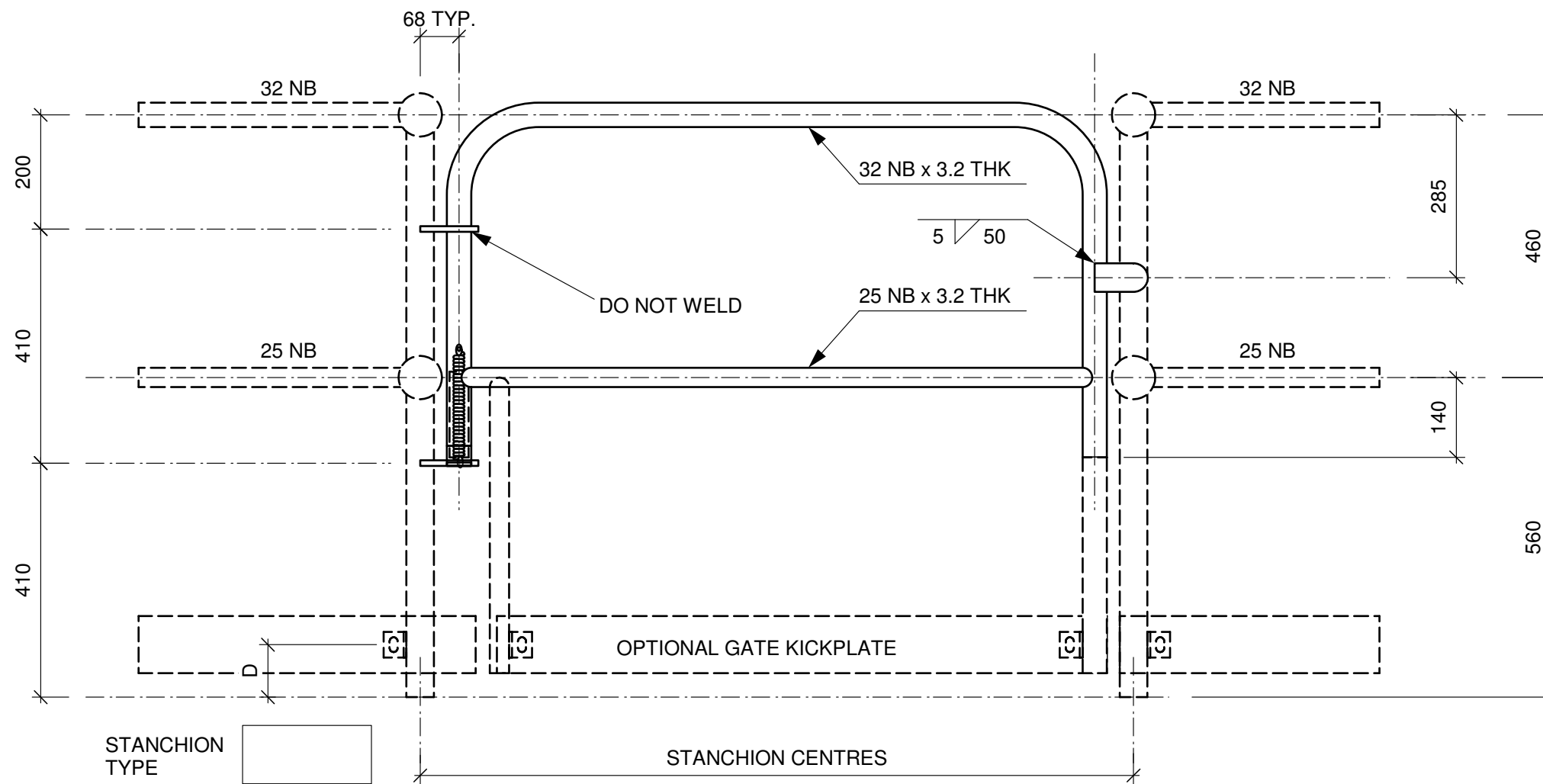
ELEVATION - SELF CLOSING GATE
