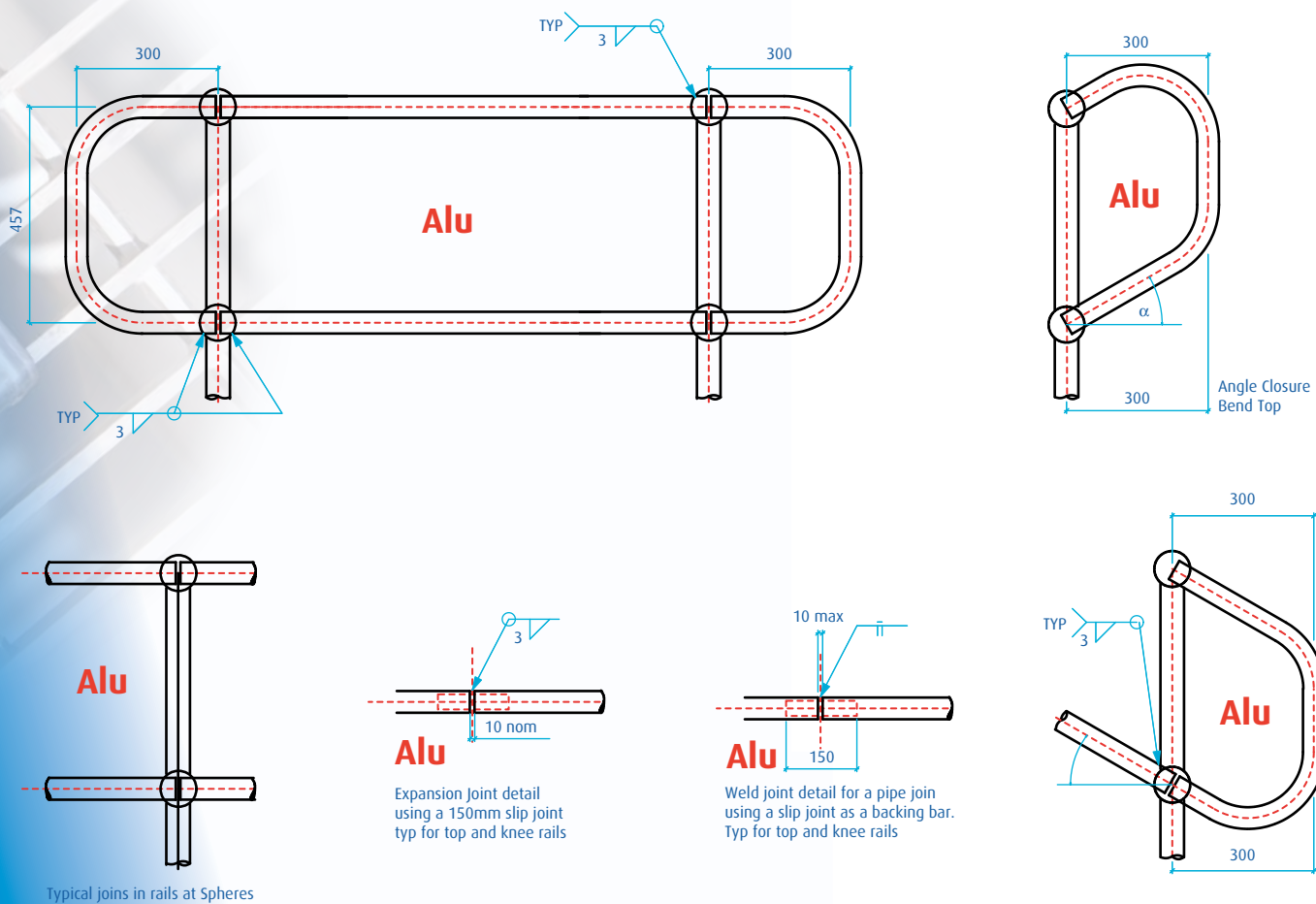
Typical joins in rails at Spheres
